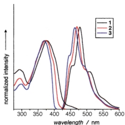
Figure 6. UV/Vis absorption (left) and fluorescence (right) spectra of 1–3 in the bulk state.
