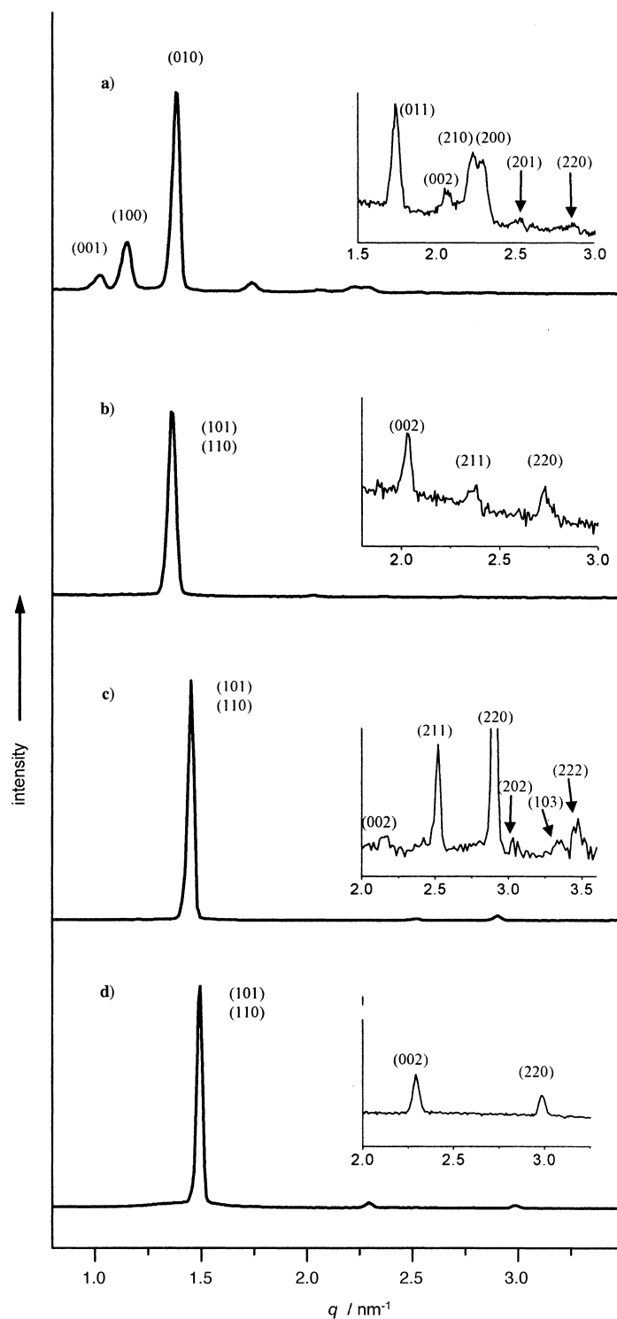
Figure 3. Small-angle X-ray diffraction patterns of a) 1 at 60^{\circ}\text{C} , b) 1 at 150^{\circ}\text{C} , c) 2 at 30^{\circ}\text{C} , and d) 3 at 30^{\circ}\text{C} .
