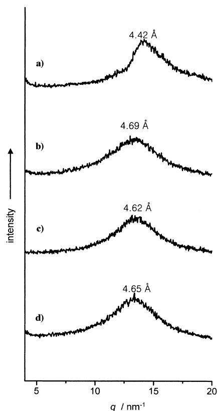
Figure 4. Wide-angle X-ray diffraction patterns of a) 1 at 30 °C, b) 1 at 150 °C, c) 2 at 30 °C and d) 3 at 30 °C.
